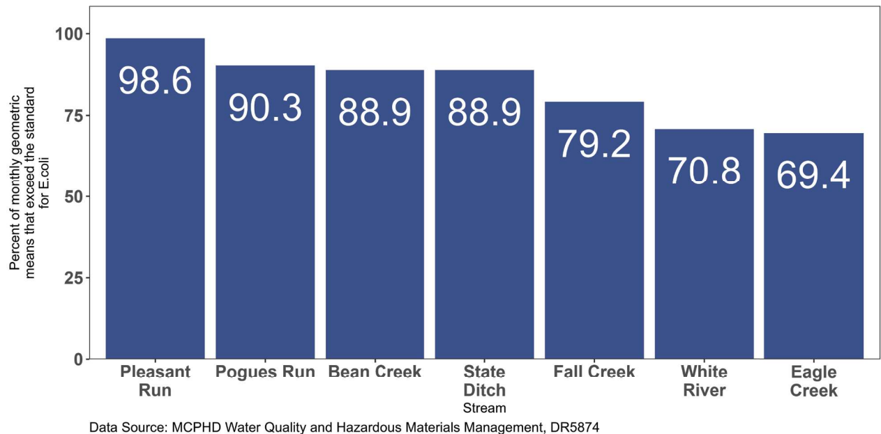
Figure 43. E. Coli in Marion County streams, 2024
